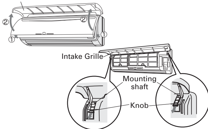
Intake Grille
